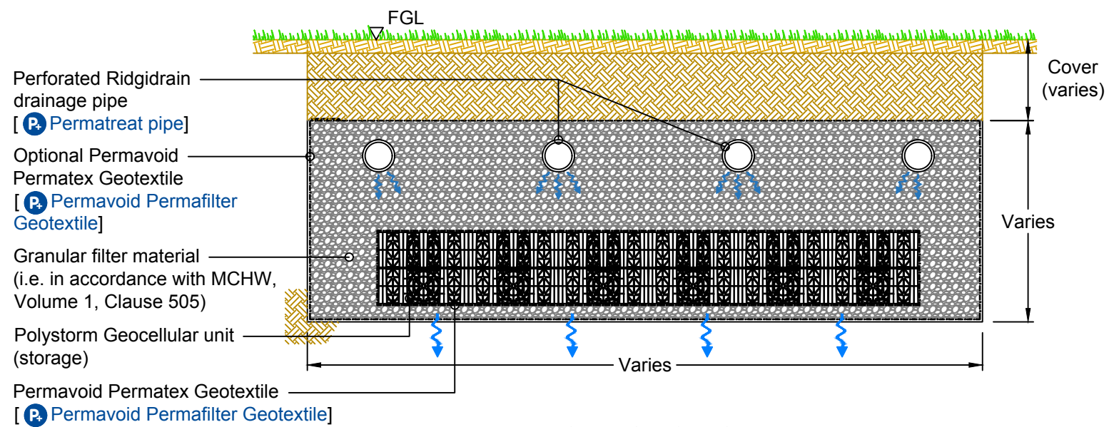
TYPICAL SECTION
