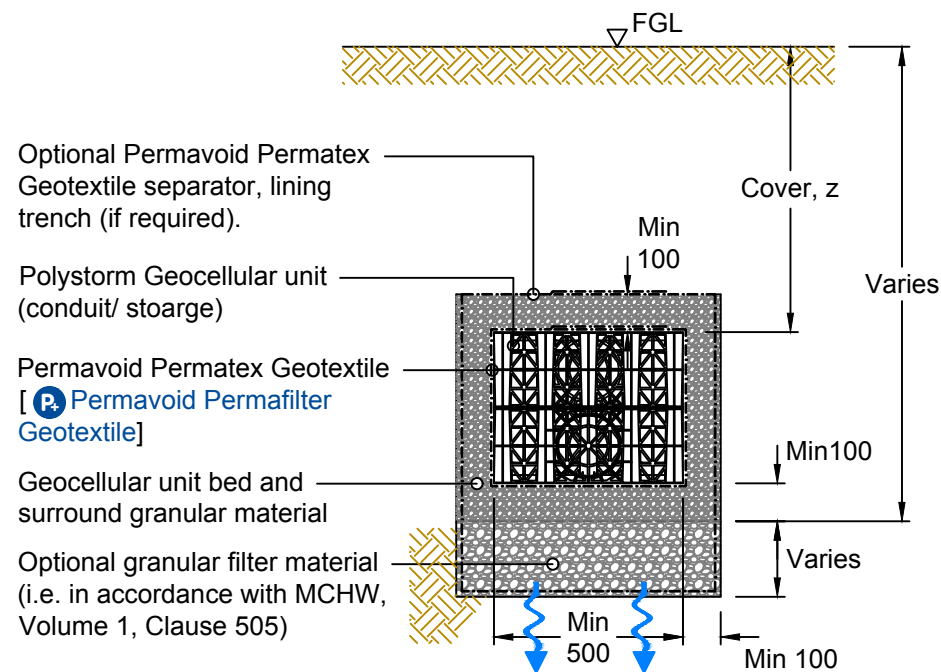
TYPICAL SECTION
