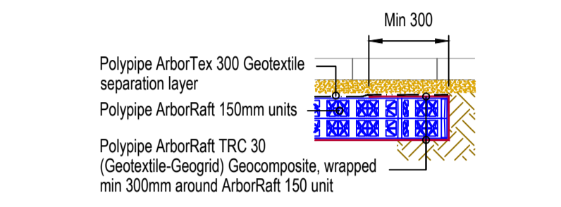
RAFT EDGE DETAIL OUTER PERIMETER NTS
