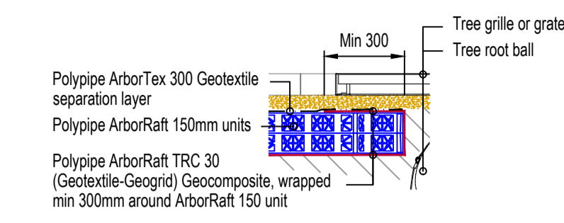
RAFT EDGE DETAIL INNER PERIMETER NTS
