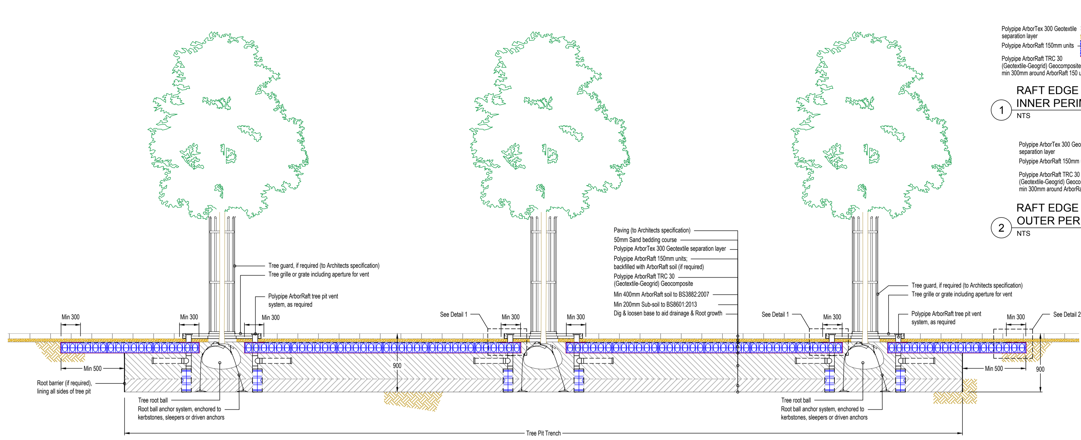
TYPICAL SECTION Scale 1:30
