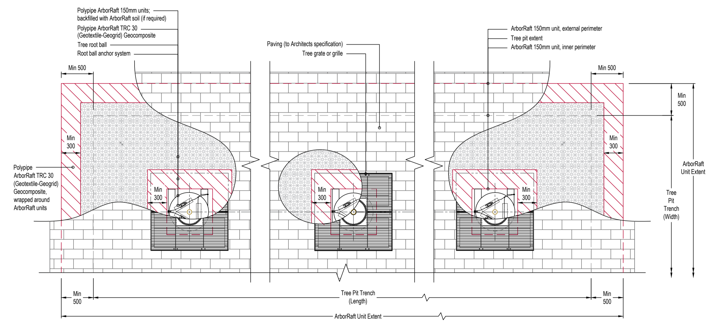
PLAN VIEW Scale 1:30
