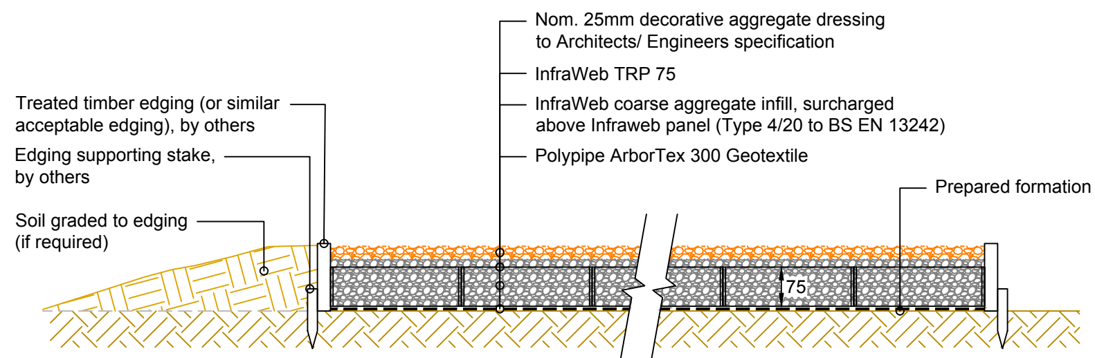
TYPICAL SECTION Scale 1:10
