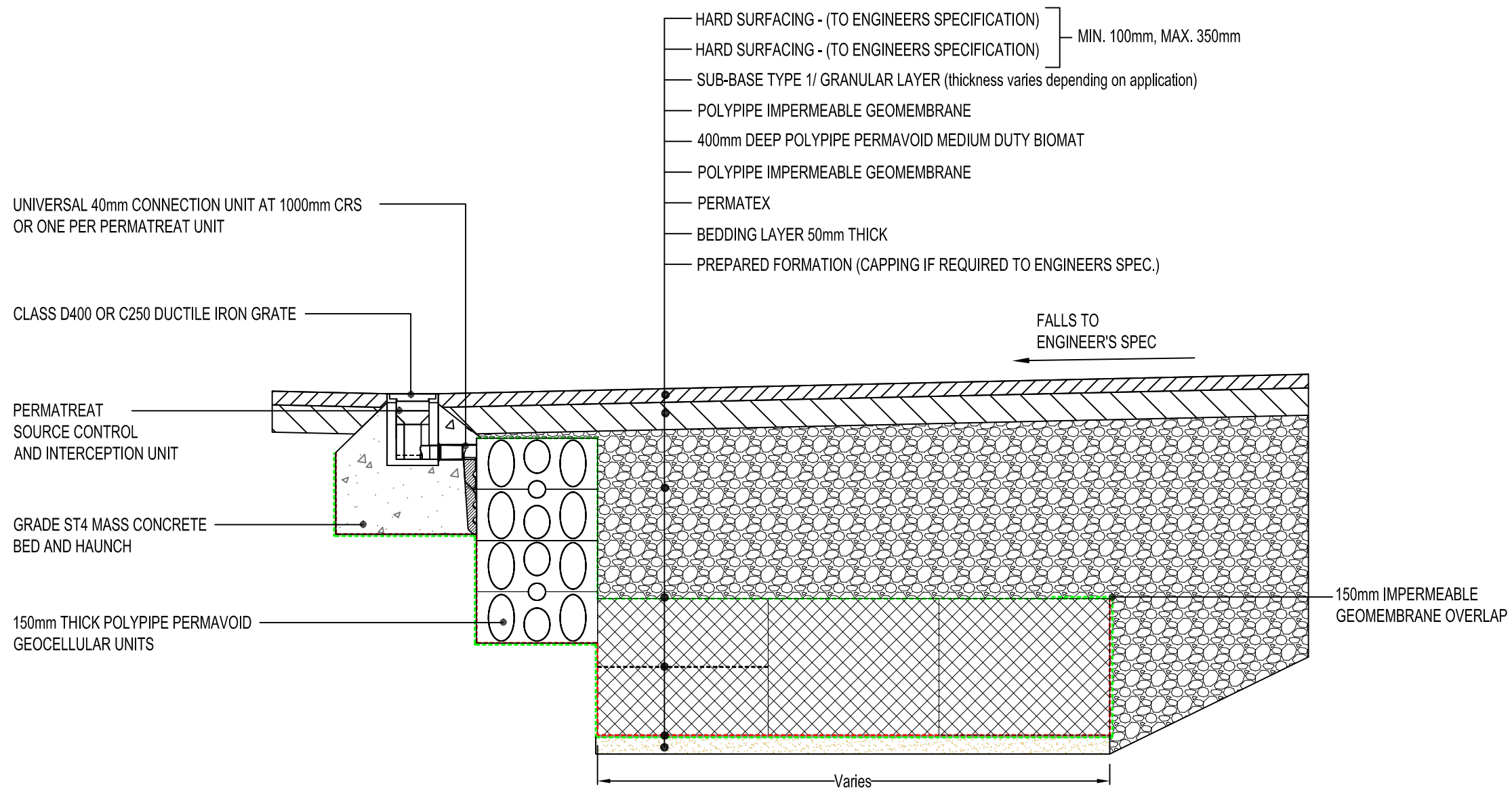
TYPICAL SECTION THROUGH POLYPIPE PERMATREAT AND PERMAVOID CONDUIT WITH POLYSTORM TREATMENT ATTENUATION TANK Scale (1:15)
