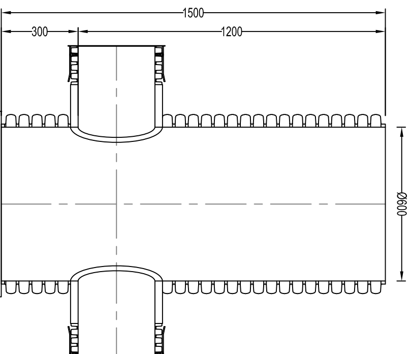
CP60015300 - SECTION A-A Scale (1:15)
