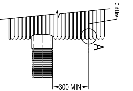
CHAMBER HEIGHT REDUCTION DETAIL Scale (1:30)
